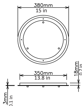
Ceiling plate
